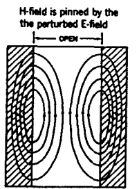
A geometry is chosen so that the oscillating H-field does not reverse sign in the open bore.
