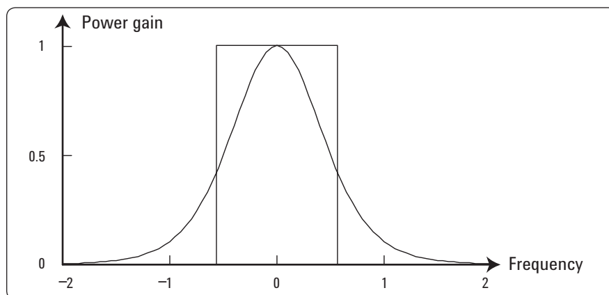
Figure 7. The power gain versus frequency of an RBW filter can be modeled by a rectangular filter with the same area and peak level, and a width of the “equivalent noise bandwidth.”
