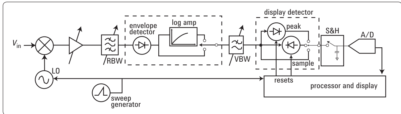
Figure A. Simplified spectrum analyzer block diagram
