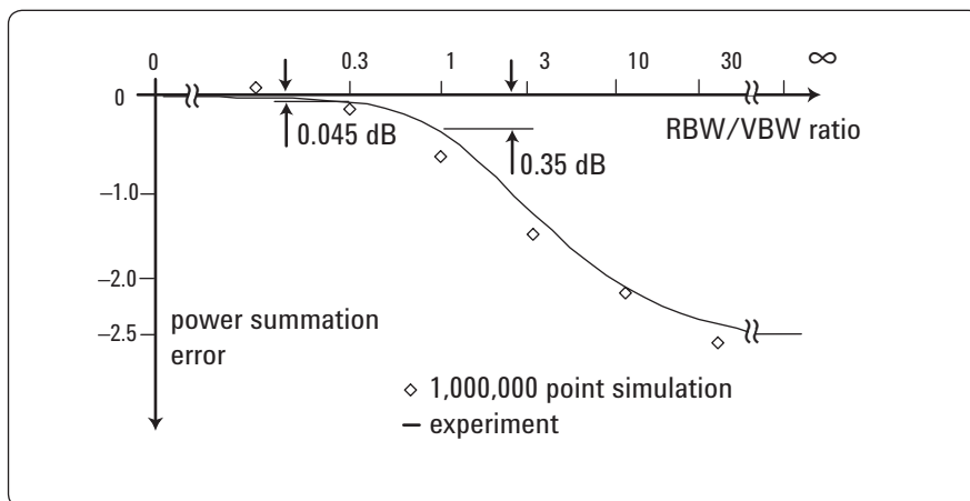
Figure 9. For \text{VBW} \geq 3\text{RBW} , the averaging effect of the VBW filter does not significantly affect power-detection accuracy.
